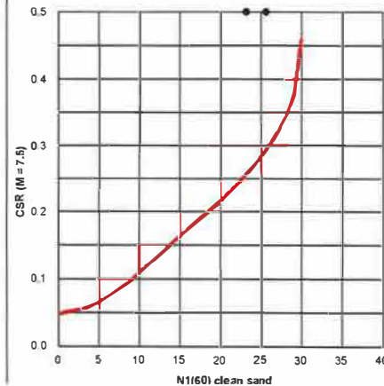
NCEER (1997) Curve of Liquefaction Resistance
