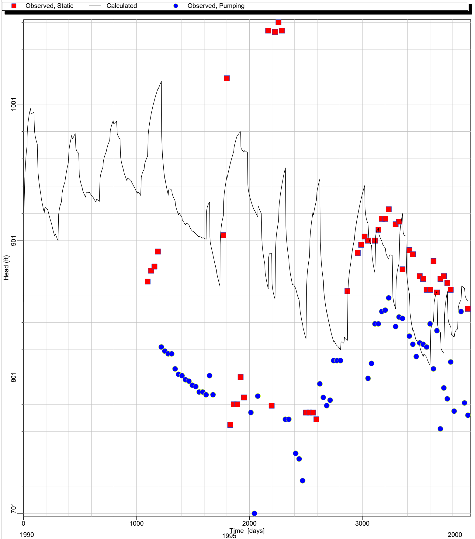
Figure E-6 - Head vs. Time (Cereal 1)
