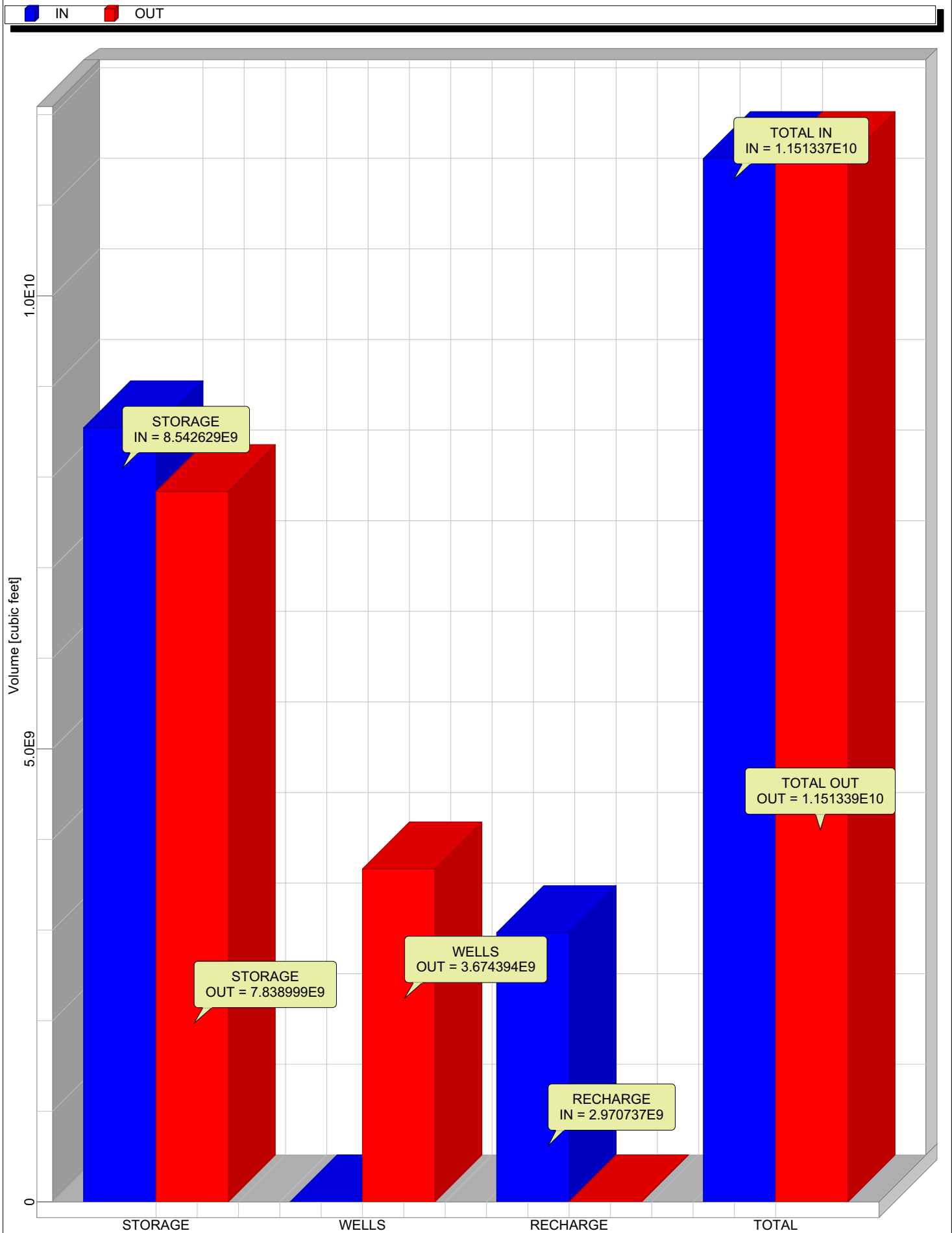
Figure E-21 - Mass Balance
