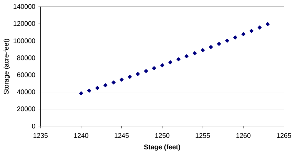
Figure F-2 Stage Storage
