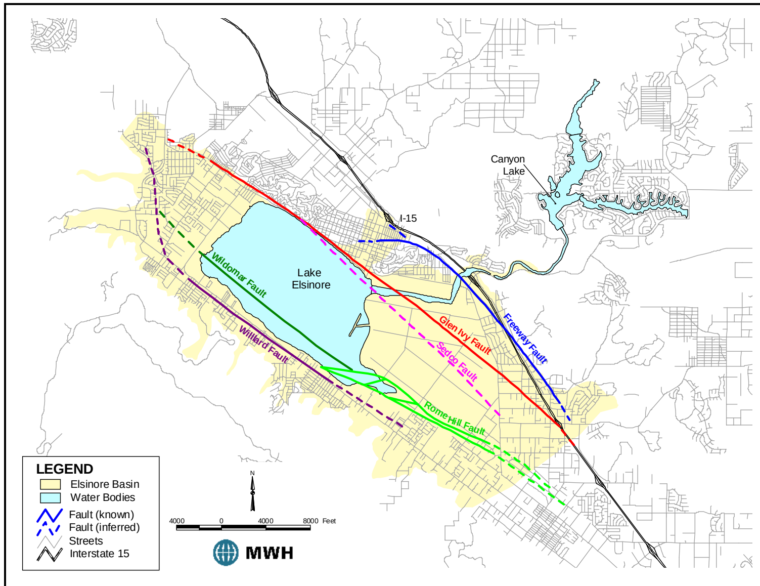
Figure 3 Faults of the Elsinore Basin
