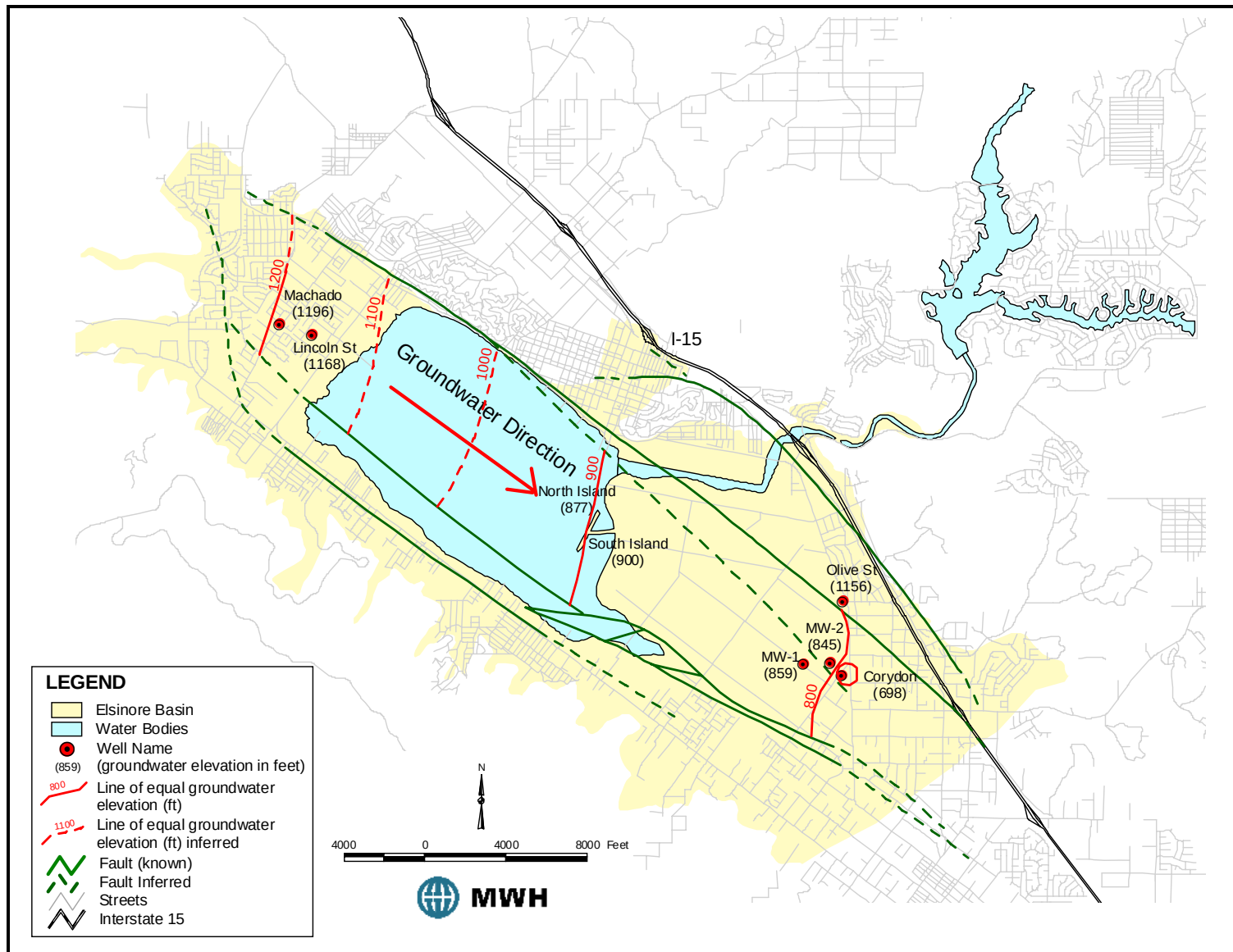
Figure 4 Groundwater Contour Map of the Fernando Group (Summer 2022)
