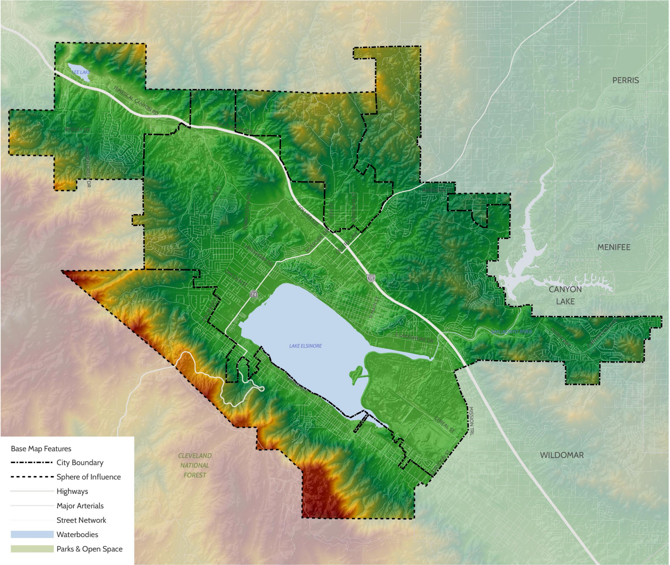
Figure 3-5 TOPOGRAPHY
